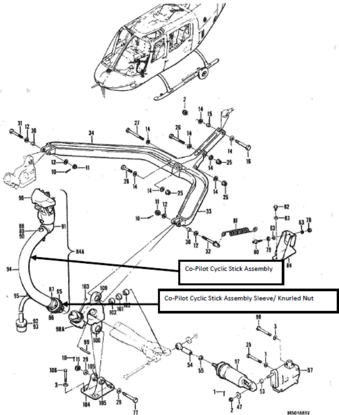
Figure 95. Control Installation, Cyclic (Sheet 2 of 2)
